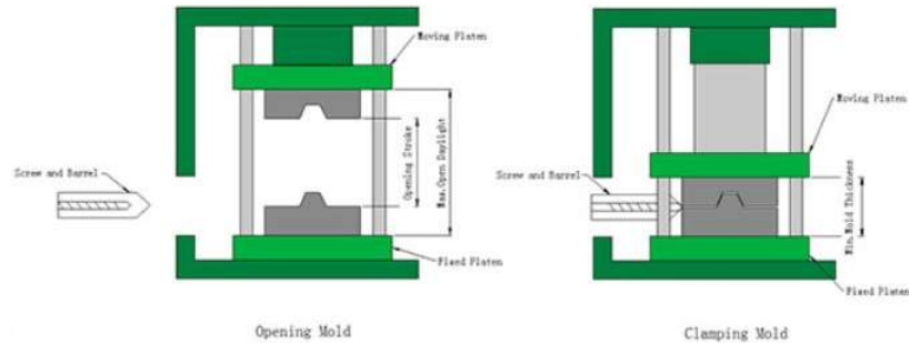
Clamping Mold
