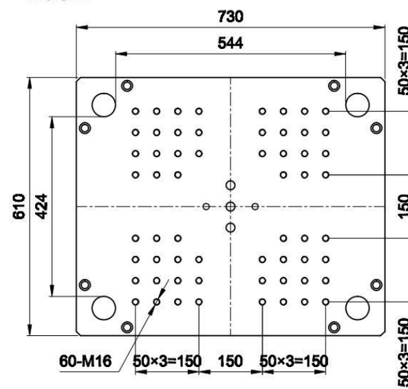
Clamping Mold
