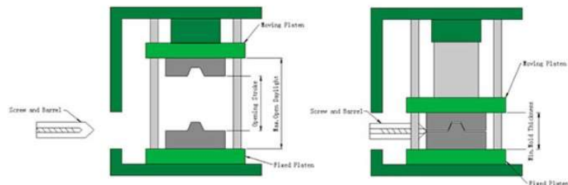
Opening Mold
