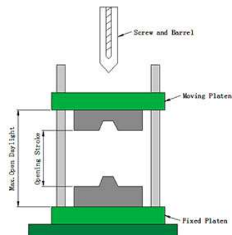
Opening Mold
