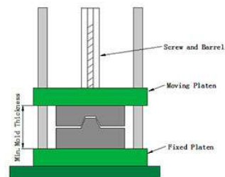
Clamping Mold
