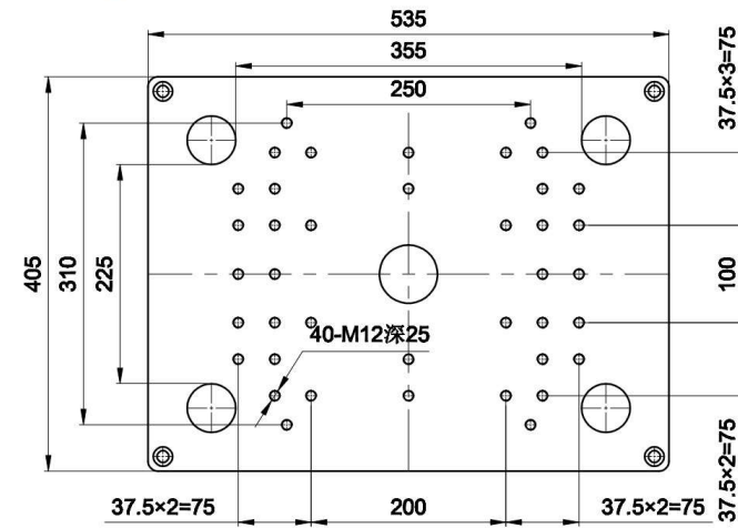
Clamping Mold
