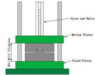
Clamping Mold
