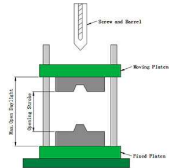
Opening Mold
