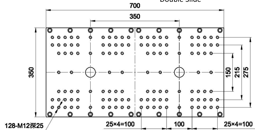
Double Slide
