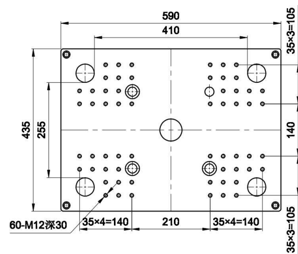
Clamping Mold
