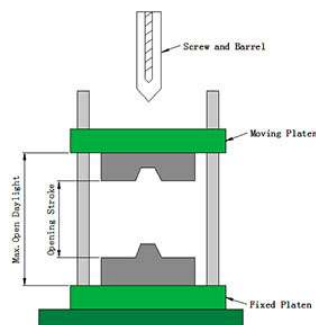
Opening Mold
