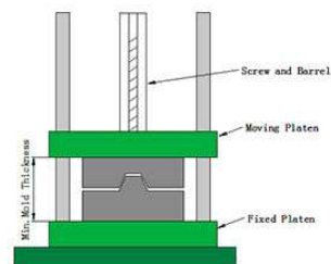
Clamping Mold
