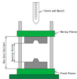
Opening Mold
