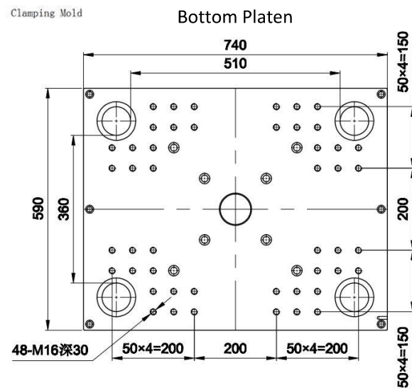
Clamping Mold
